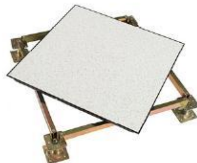
有横梁地板及支架安装 installation: panel, pedestal and stringer
