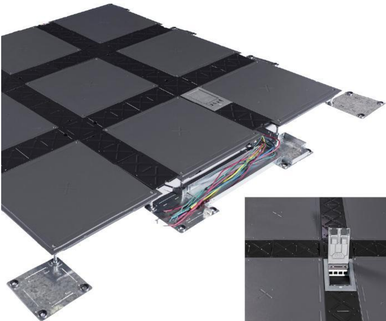
地板、地插座、专用线槽安装 installation: panel, socket and trunking
